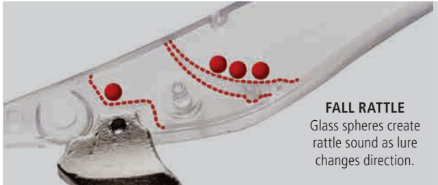
FALL RATTLE Usually Egi only rattle when they are twitched and jerked. The Clinch Rattle series is equipped with the original 'rattle system', which produces sound when falling in a straight or curved trajectory.
